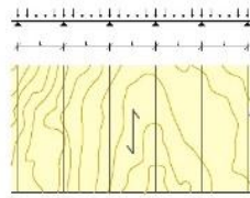
Grain direction perpendicular to the span (I-)
