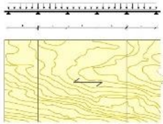
Grain direction parallel to the span (II)
