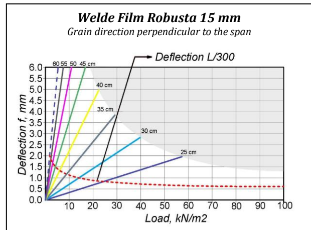
Grain direction perpendicular to the span (I-)
