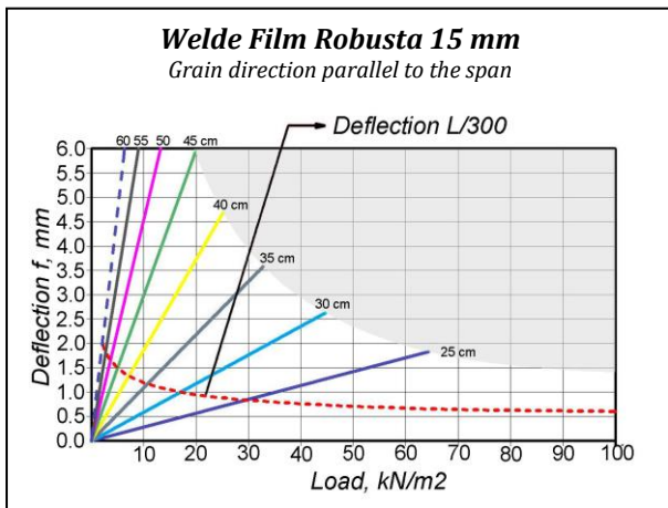
Grain direction parallel to the span (II)
